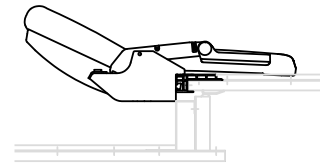
Folded Citation chair
